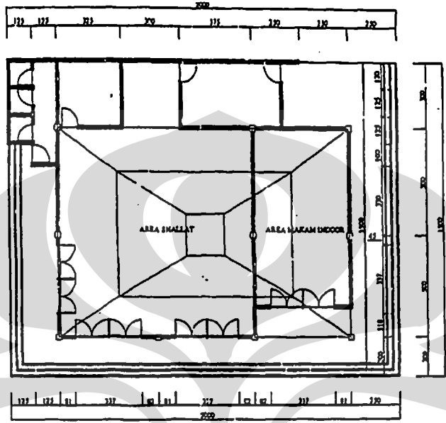
DENAH MUSTIOLA
