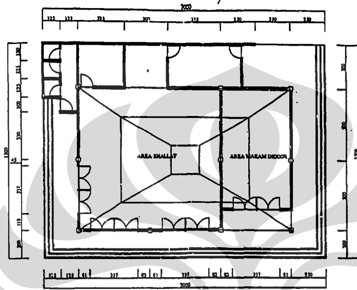
DENAH MUSHOLA
