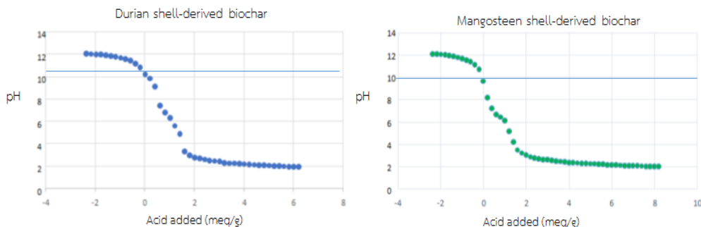
Fig. 1. pH titration curves for durian shell-derived biochar and mangosteen shell-derived biochar.
