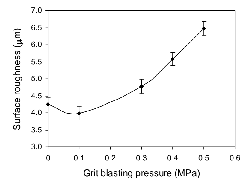
Figure 1 Effects of grit blasting pressure on the surface roughness
