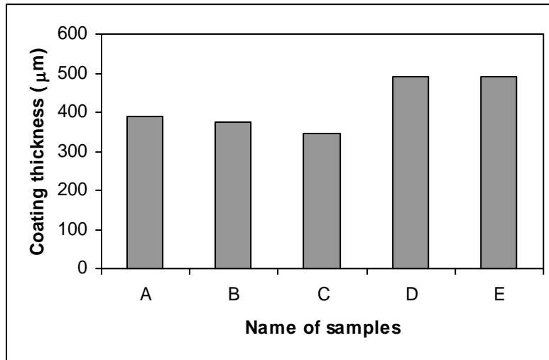
Figure 2 Variety of WC-Co coating thickness on samples with different surface roughness. Sample A: without grit blasting, and other samples with grit blasting with the pressure of: B: 0.1 MPa, C: 0.3 MPa, D: 0.4 MPa and E: 0.5 MPa
