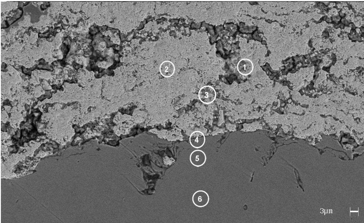
Figure 5 SEM micrograph of the coating - substrate interface region
