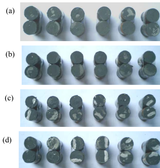
Figure 3 Fracture surfaces of adhesion test samples with grit blasting pressure of (a) 0.1 MPa, (b) 0.3 MPa, (c) 0.4 MPa and (d) 0.5 MPa. The dark surface is the fracture occurs within the epoxy layer, while the light surface is the fracture occurs between the epoxy and the WC-Co coating
