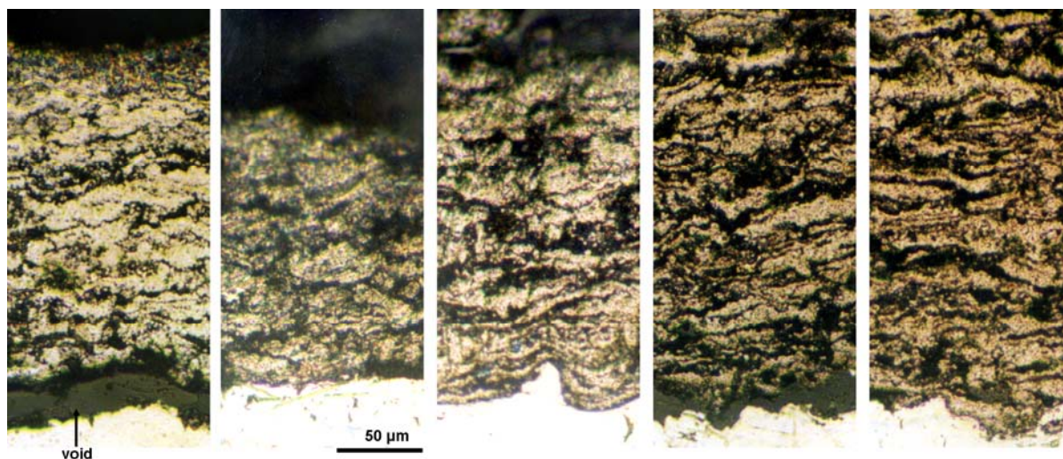
Figure 4 Micrographs of WC-Co coating on samples with grit blasting pressure of (a) 0 MPa (without grit blasting), (b) 0.1 MPa, (c) 0.3 MPa, (d) 0.4 MPa and (e) 0.5 MPa
