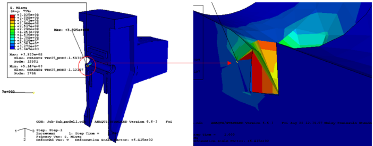
Figure 10 Von Misses result of sub-modeling technique without cyclic loading
