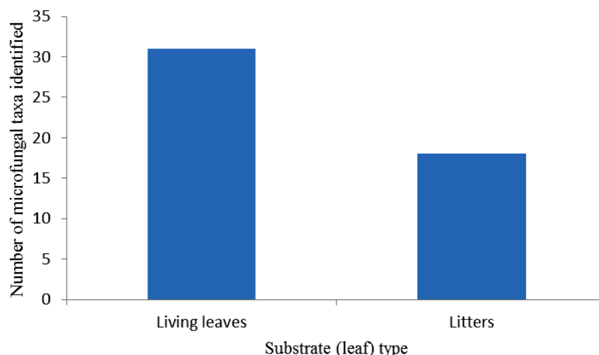
Figure 1. Microfungi Taxa Identified on Living Leaves and Litters of L. bidentata
