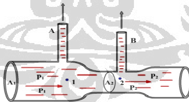
Gambar 2.3. Venturi
