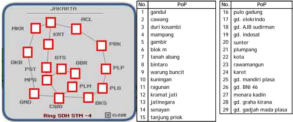
Gambar L- 57 Ring Metro Ethernet over NG SDH ICON+
