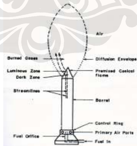
Gambar 2.1 Bunsen burner
