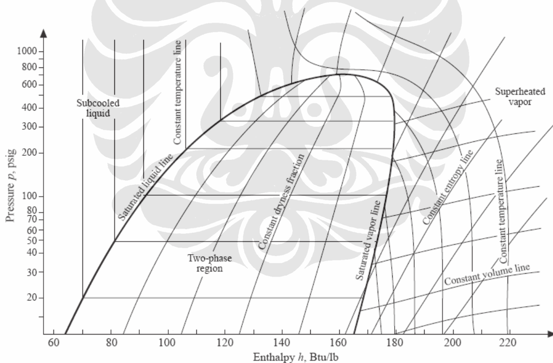
Gambar 2.1 Diagram tekanan-entalpi [2]
