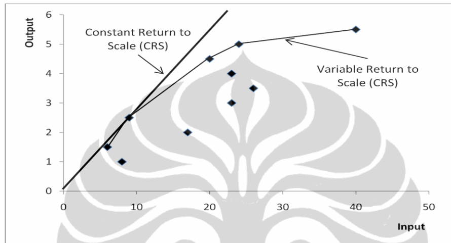
Gambar 2.4. Model DEA Constant Return to Scale dan Variable Return to Scale
