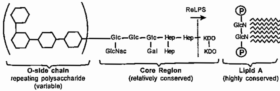
Figure 2. Lipopolysaccharide structure 15
