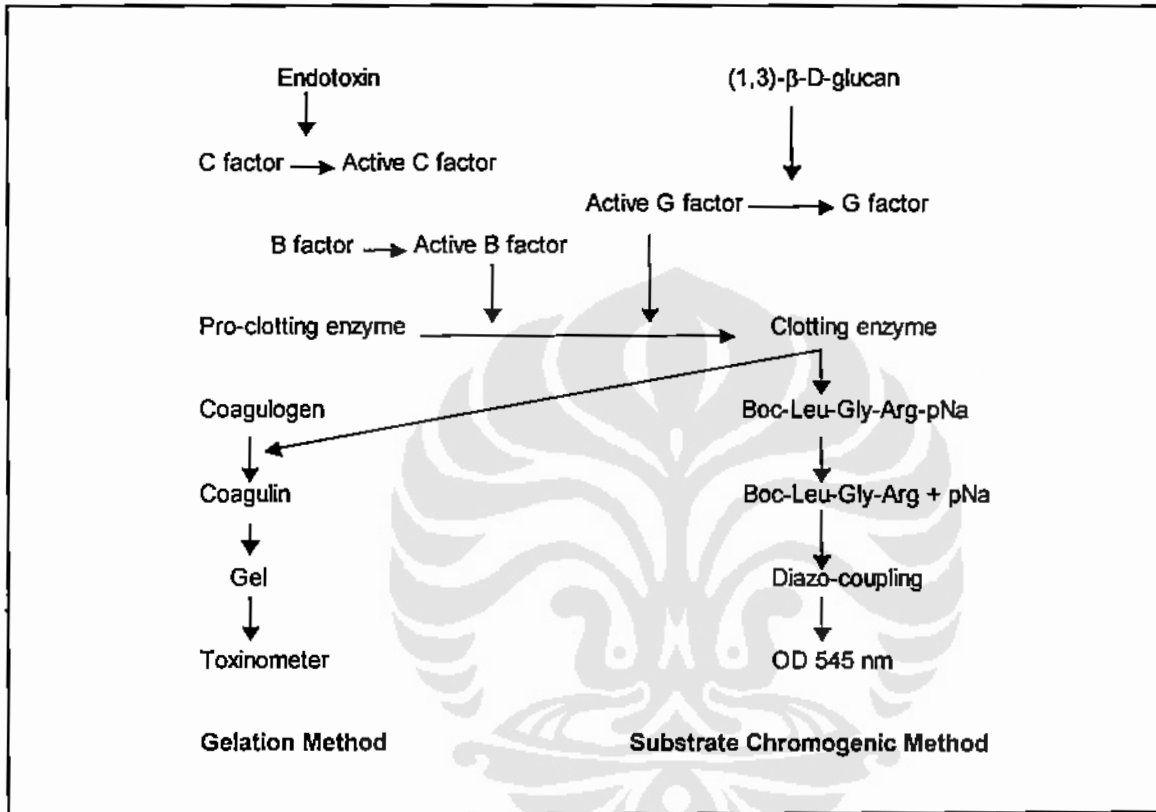
Figure 5. The principle of limulus evaluation
