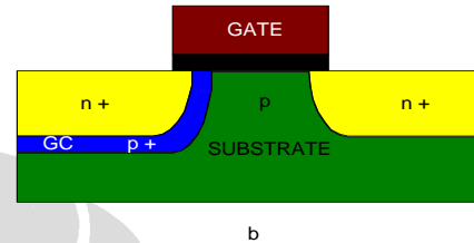
Gambar 1. Struktur divais (a) CMOS ungraded , (b) GCMOSFET unilateral
