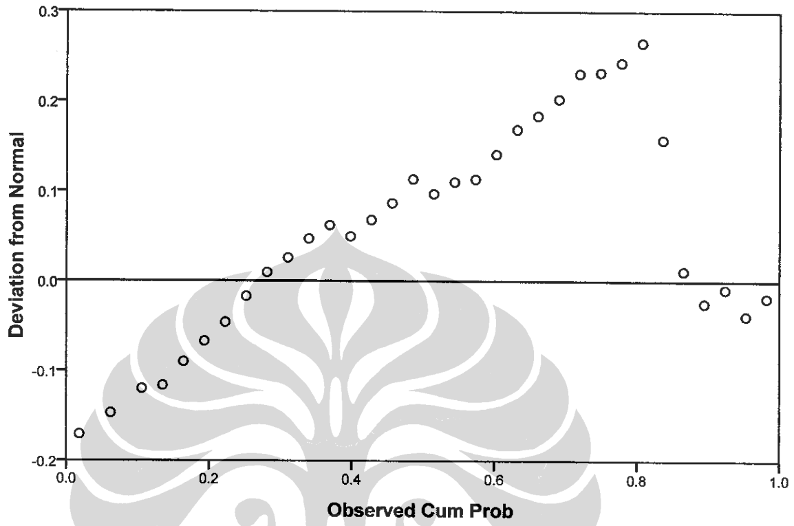
Detrended Normal P-P Plot of ROAX1
