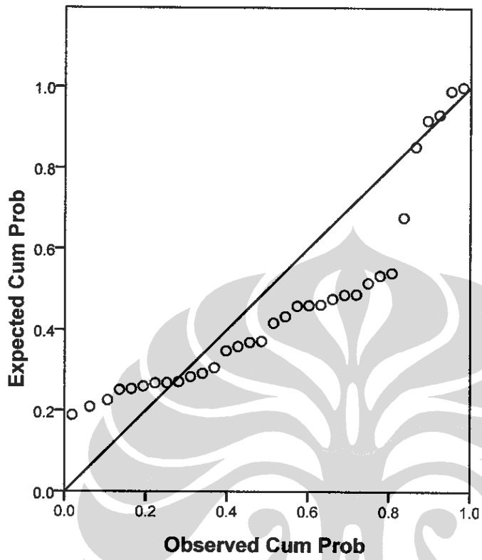
Normal P-P Plot of ROAX1
