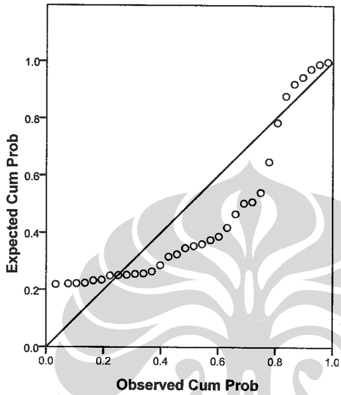
Normal P-P Plot of EPSX2
