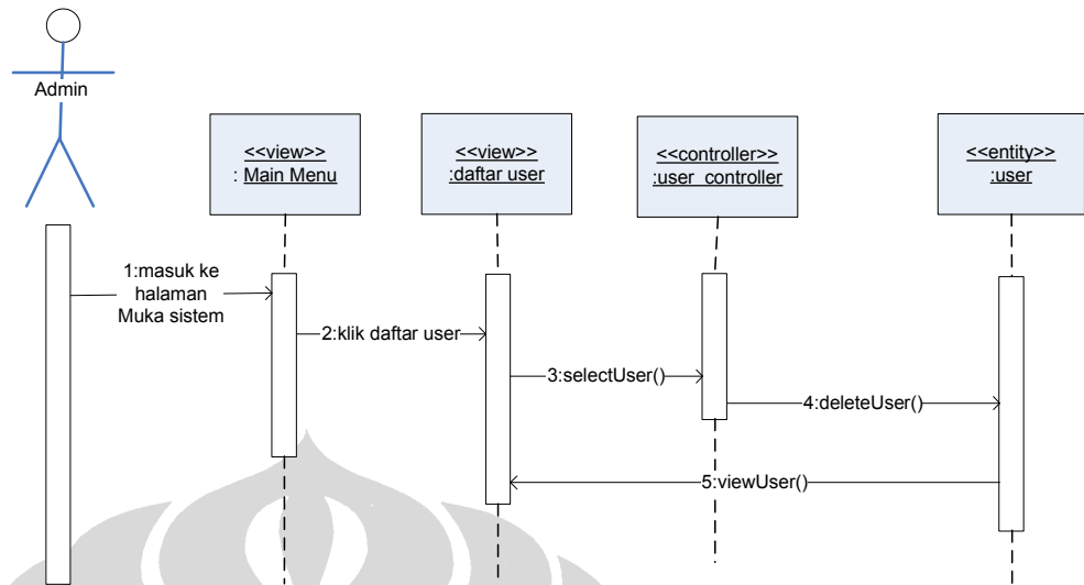
Gambar 60. Sequence diagram untuk use case delete User
