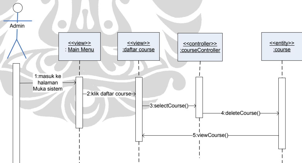
Gambar 61. Sequence diagram untuk use case delete Course
