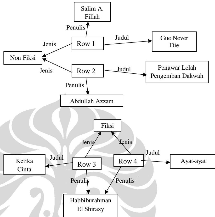
Gambar 3.5 RDF Graph
