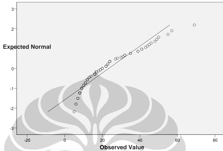
Normal Q-Q Plot of Umur
