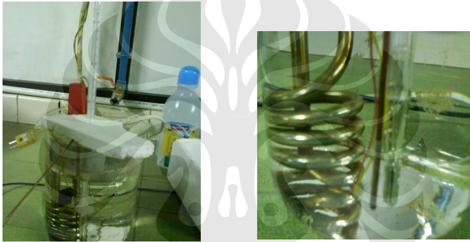
Gambar IV.10 Kalibrasi termokopel
