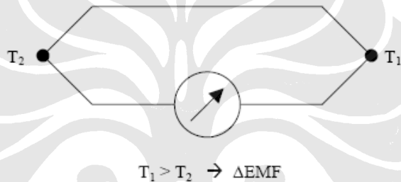
Gambar IV. 8 Termokopel
