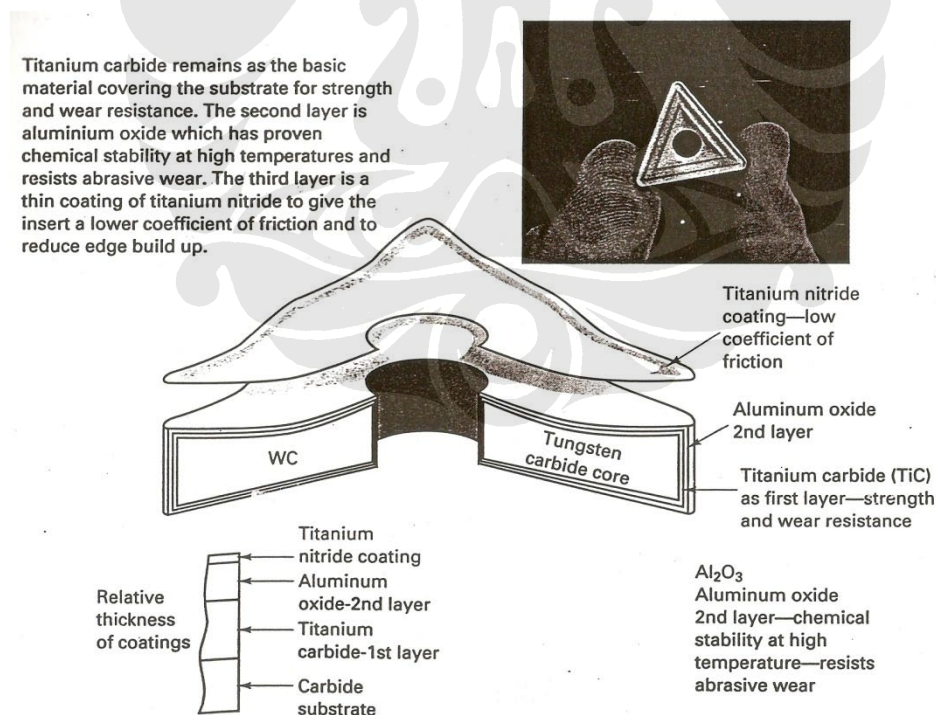
Gambar IV.5 CVD-Coated Carbide [6]
