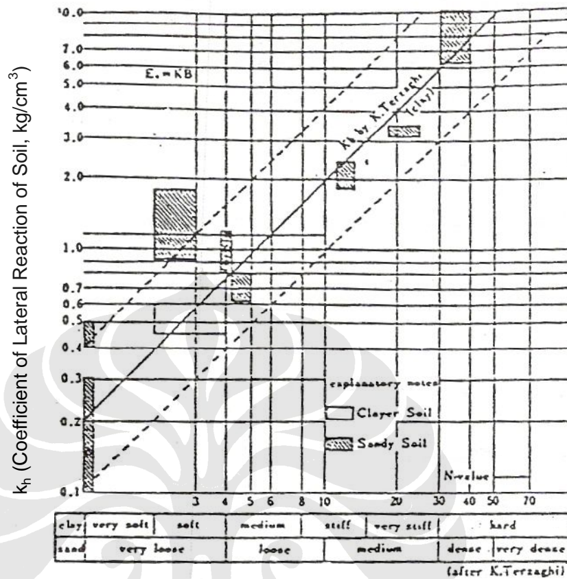
Gambar 2. 10 Nilai k_h Berdasarkan Yokohama (Sumber: Steel Sheet Piling Design Manual )
