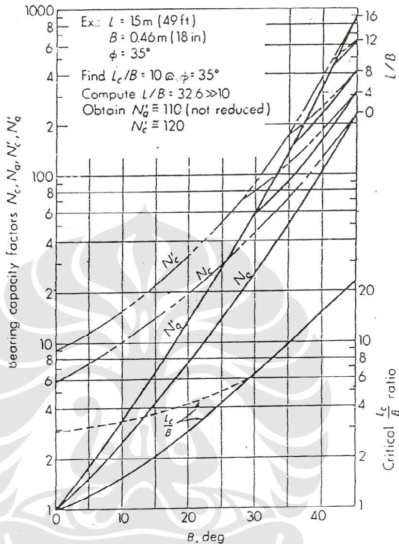
Gambar 2. 9 Bearing Capacity Factors N_c, N_q (Meyerhof)
