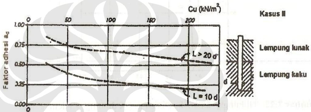
Gambar 2. 8 Faktor Adhesi (α) (Tomlinson)
