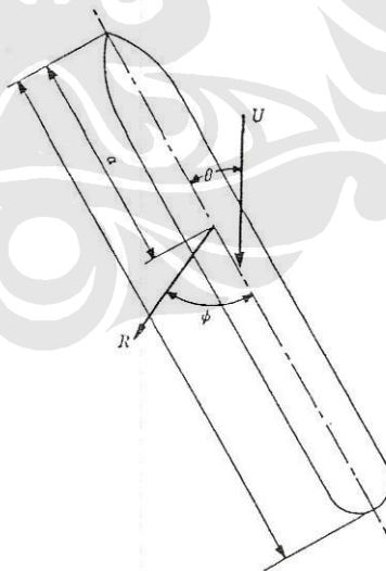
Gambar 2. 4. Diagram Perhitungan Tekanan Angin (Sumber: Technical Standards For Port And Harbour Facilities In Japan )
