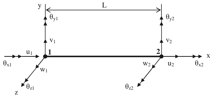
Gambar 2. 15 DOF Lengkap Element Frame (Space Frame)
